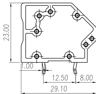
WITHOUT COVER
